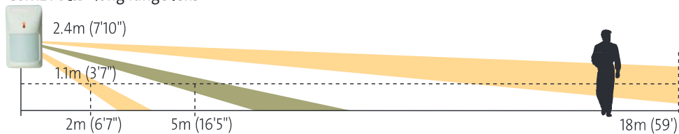
CoMET PIR - long range lens
